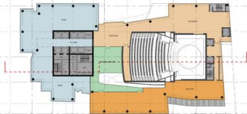
LEVEL 2 PLAN
